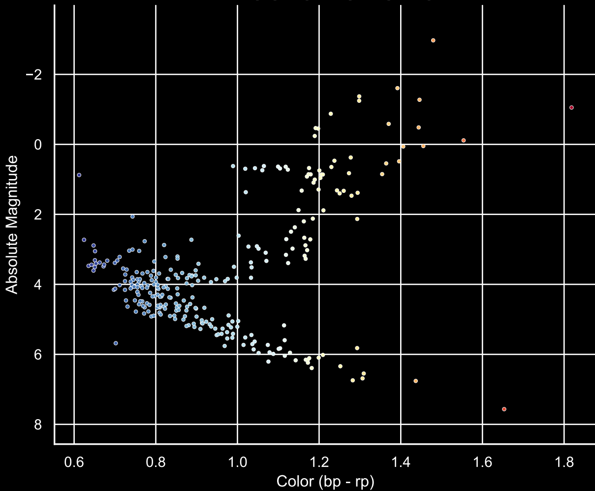
GALAH Hertzprung-Russel Diagram Field [52] Ra [329.29] Dec [-62.49]
