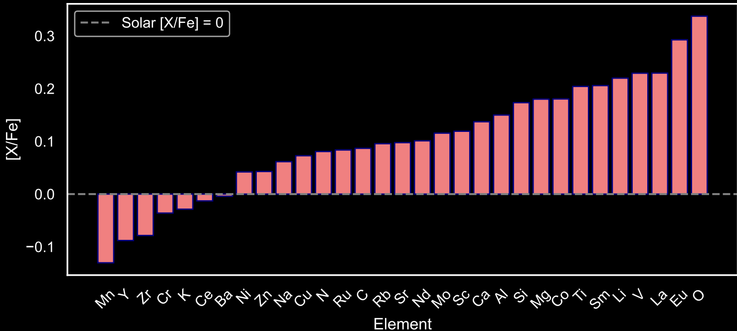
Abundance Pattern for GALAH Red Giants: Star Field [52] (N=71)
