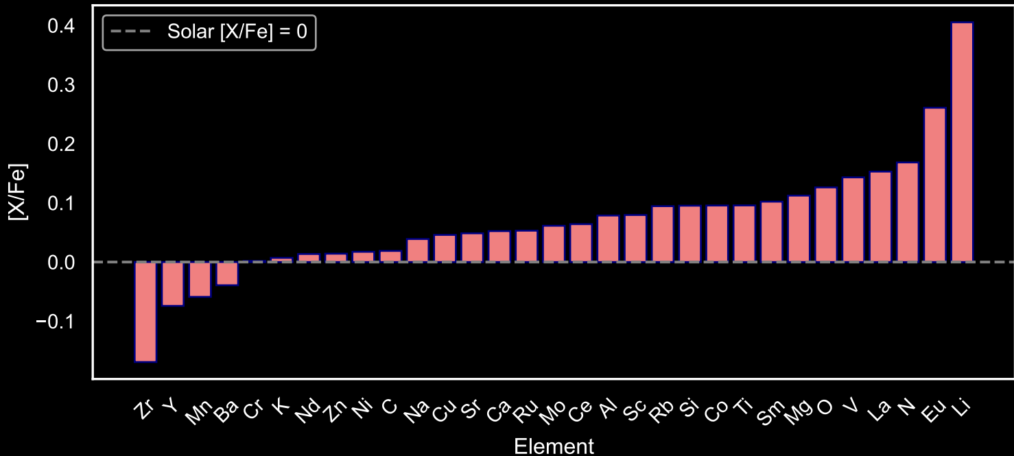
Abundance Pattern for GALAH Star Field [52] (N=287)
