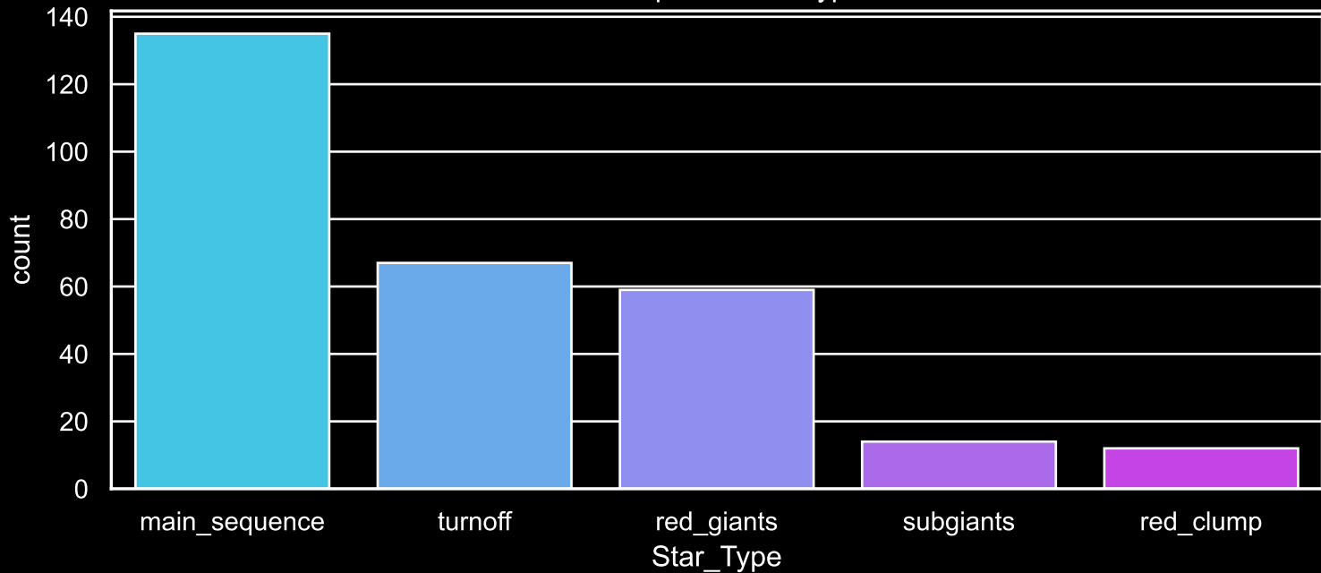
Field [52] Count plot of Star Type
