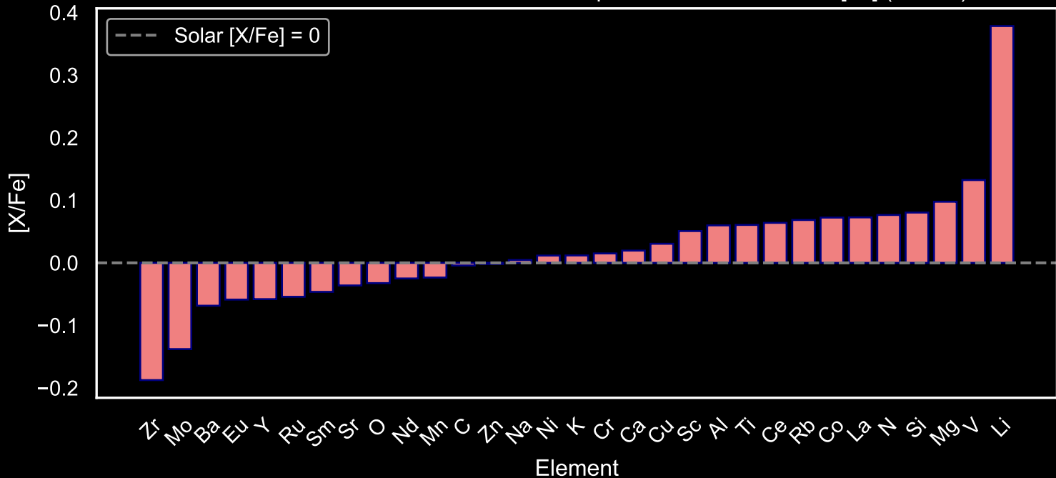
Abundance Pattern for GALAH Main Sequence Stars: Star Field [52] (N=135)
